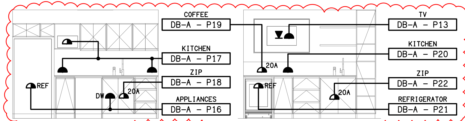
DETAIL A STAFF ROOM ELEVATION SCALE 1:50
